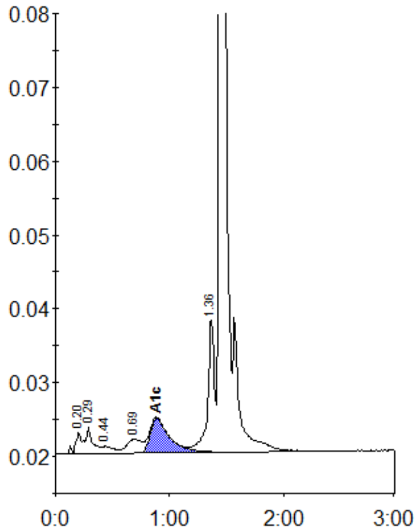
Peak table - ID: 11649200
