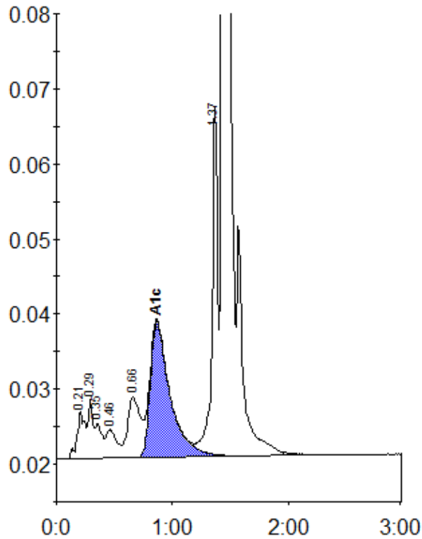
Peak table - ID: 11517569
