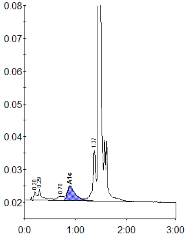
Peak table - ID: 11656336
