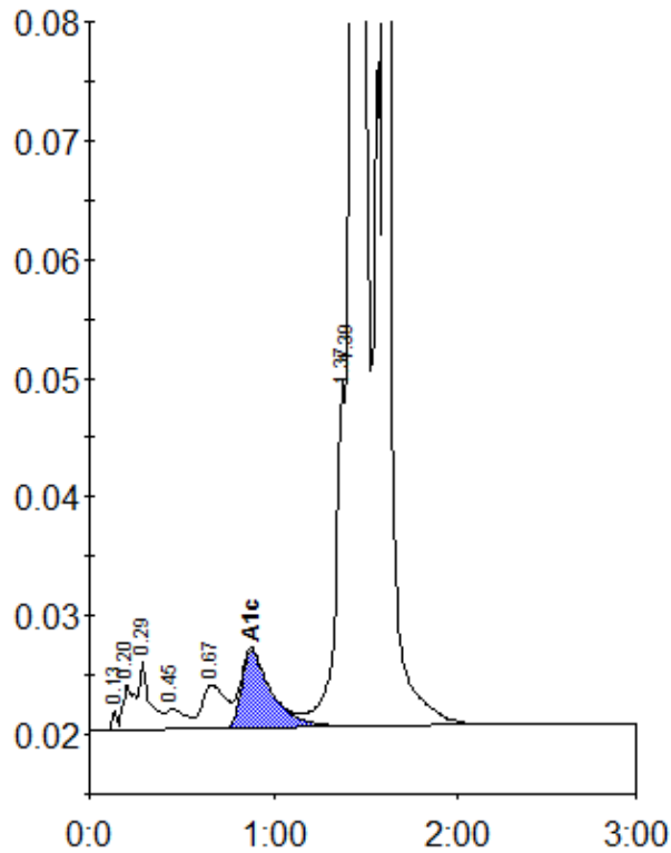
Peak table - ID: 11642341
