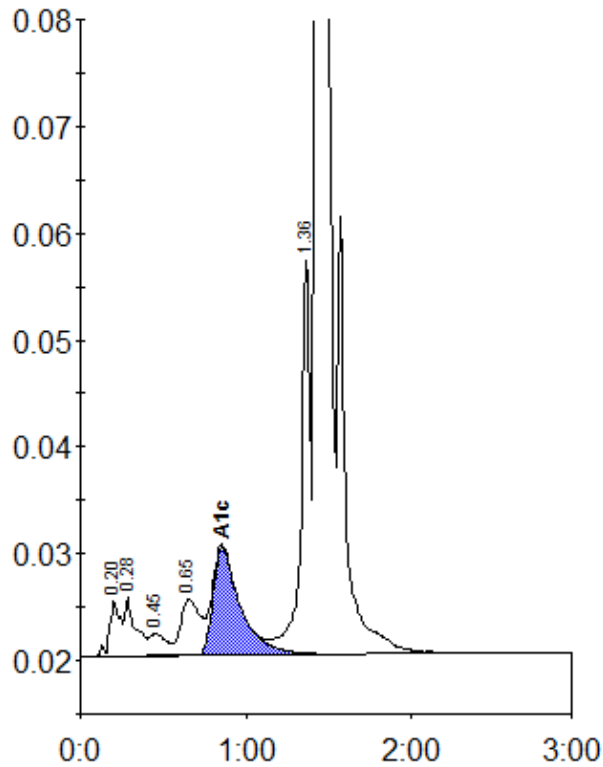
Peak table - ID: 11646302
