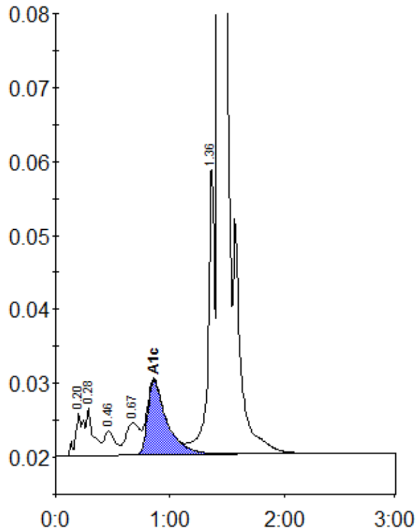
Peak table - ID: 11796998
