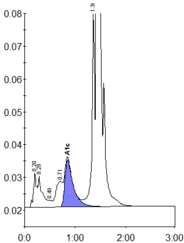
Peak table - ID: 11668783
