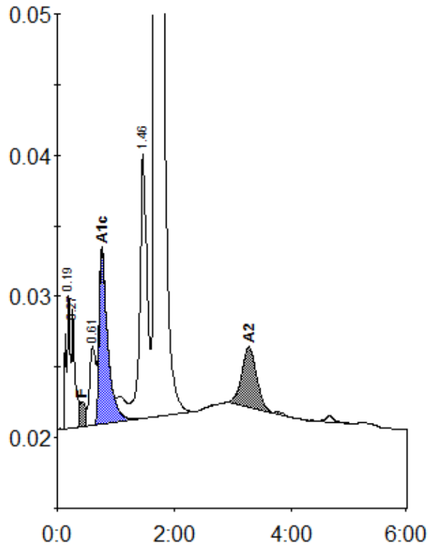
Peak table - ID: 11794667
