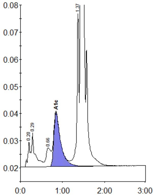
Peak table - ID: 11501893
