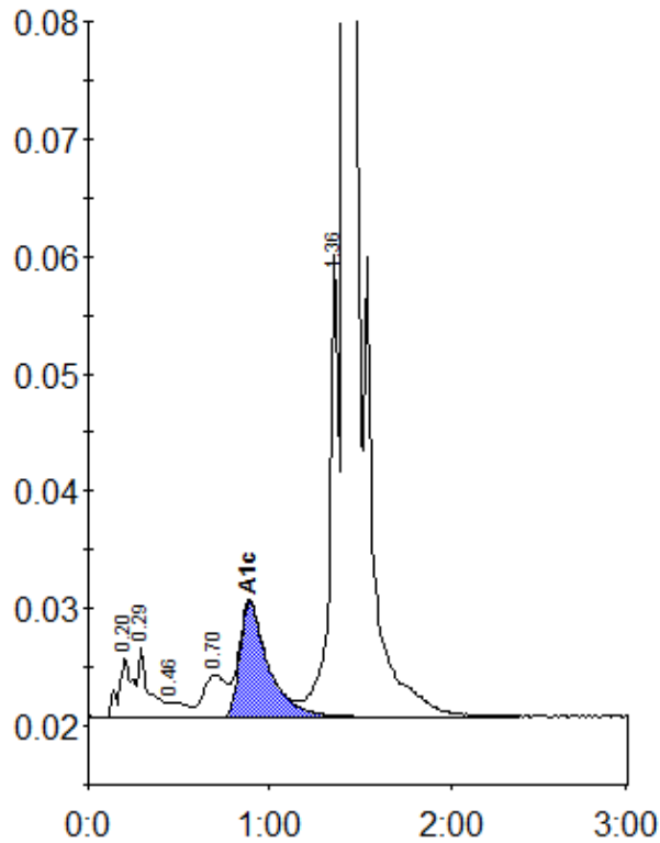
Peak table - ID: 11654633
