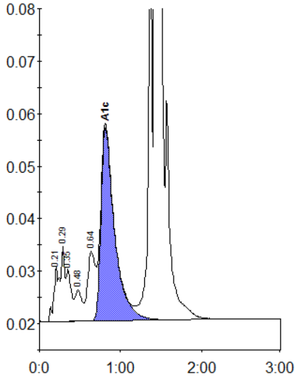
Peak table - ID: 11657449
