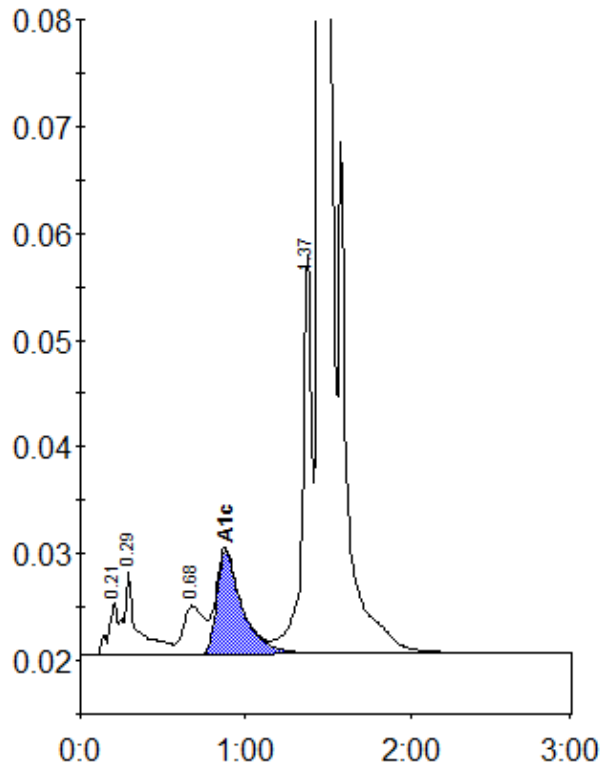
Peak table - ID: 11527116
