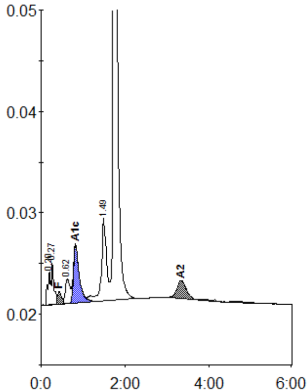
Peak table - ID: 11665890
