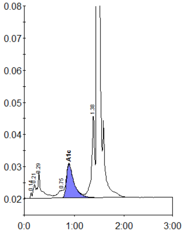
Peak table - ID: 11643676
