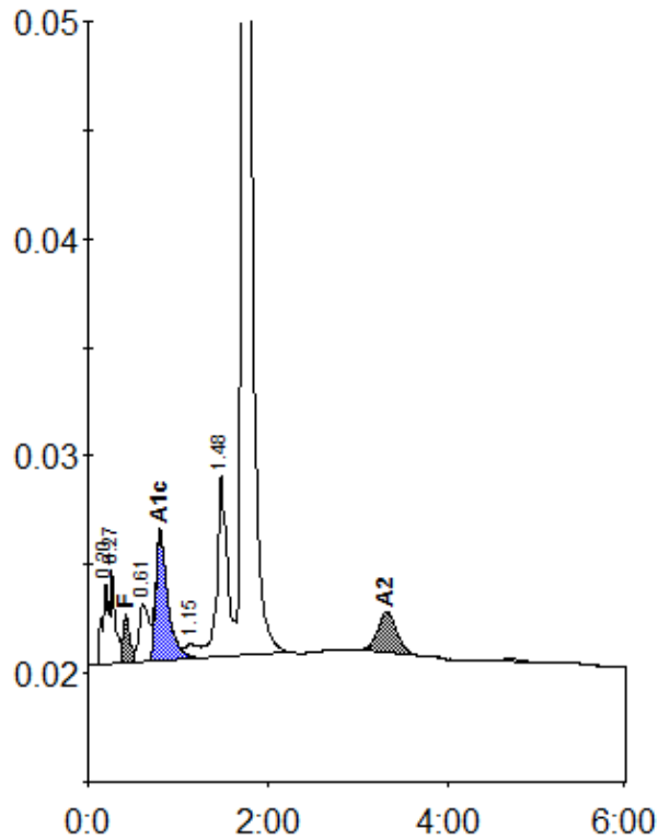
Peak table - ID: 11662665
