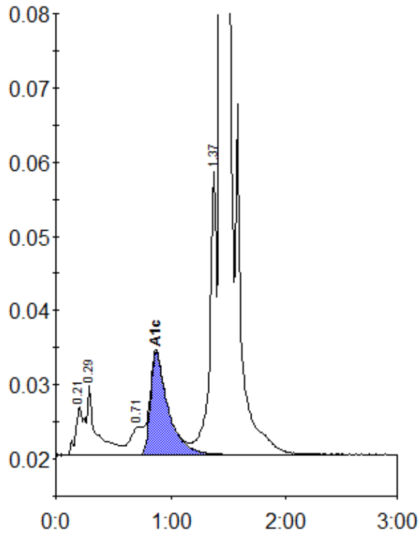
Peak table - ID: 11643687
