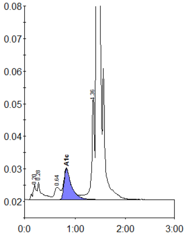
Peak table - ID: 11643494
