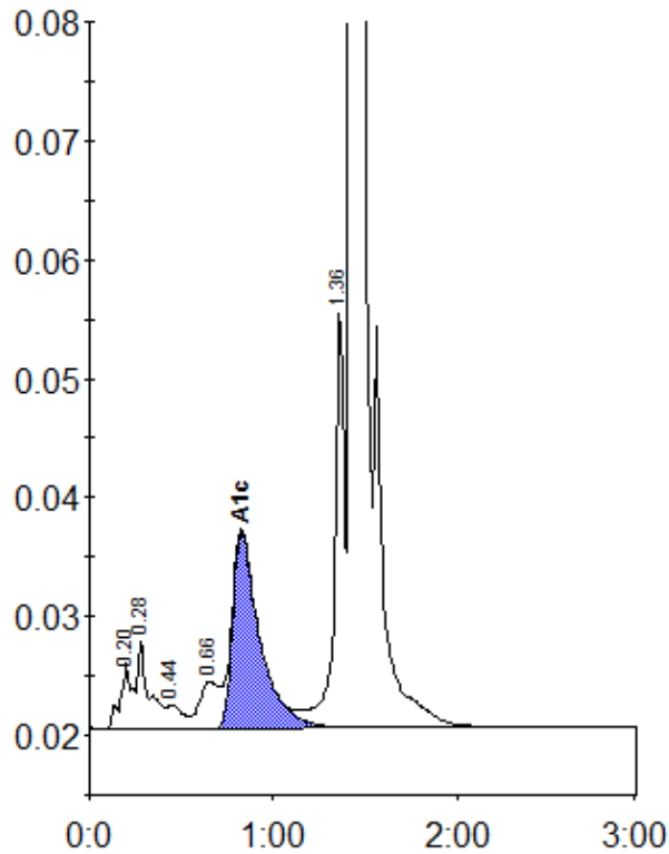
Peak table - ID: 11643188
