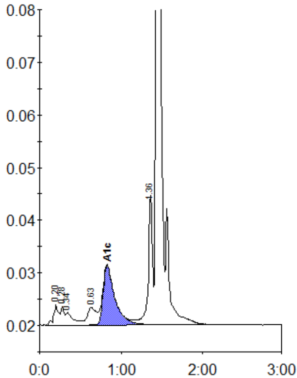
Peak table - ID: 11527275
