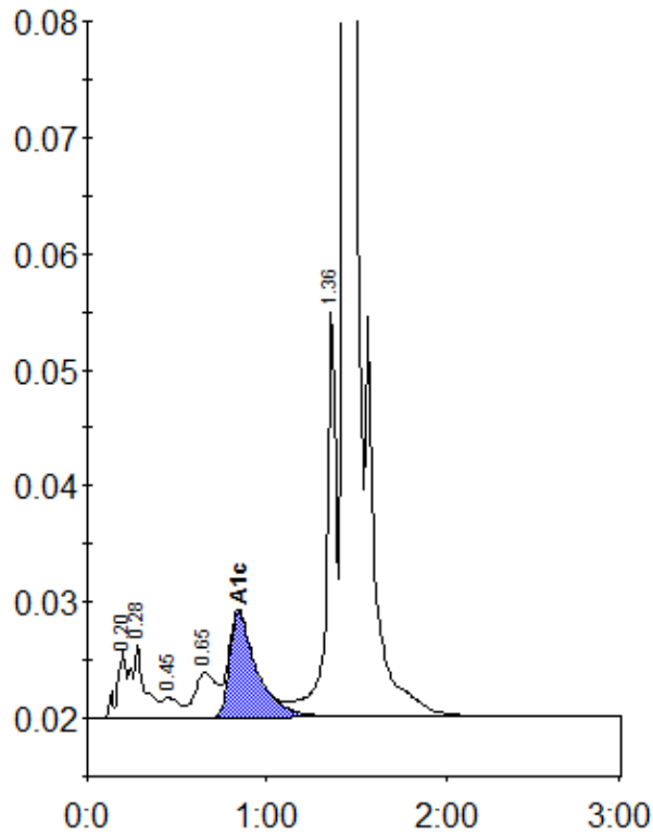
Peak table - ID: 11669201
