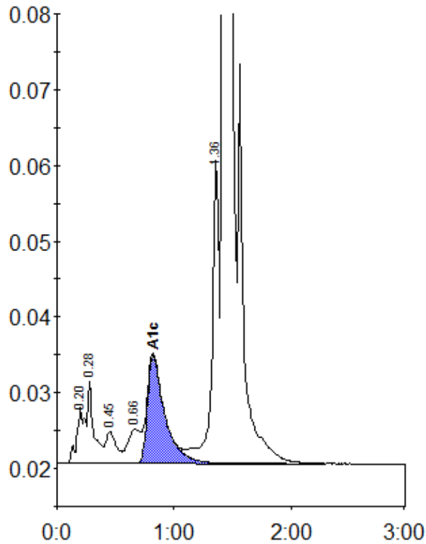
Peak table - ID: 11643790
