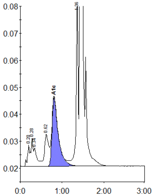
Peak table - ID: 11649661
