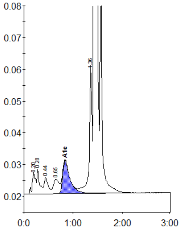
Peak table - ID: 11670706
