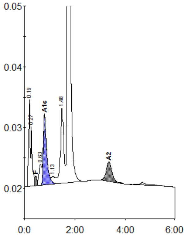
Peak table - ID: 11636071
