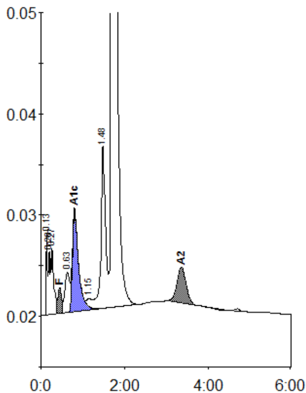
Peak table - ID: 11649513
