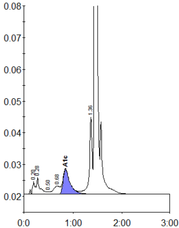
Peak table - ID: 11648289
