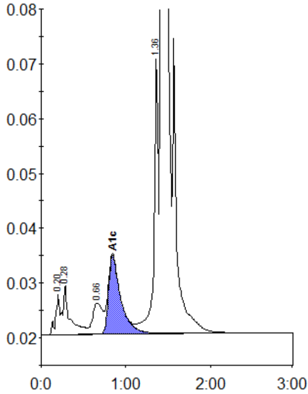
Peak table - ID: 11193703
