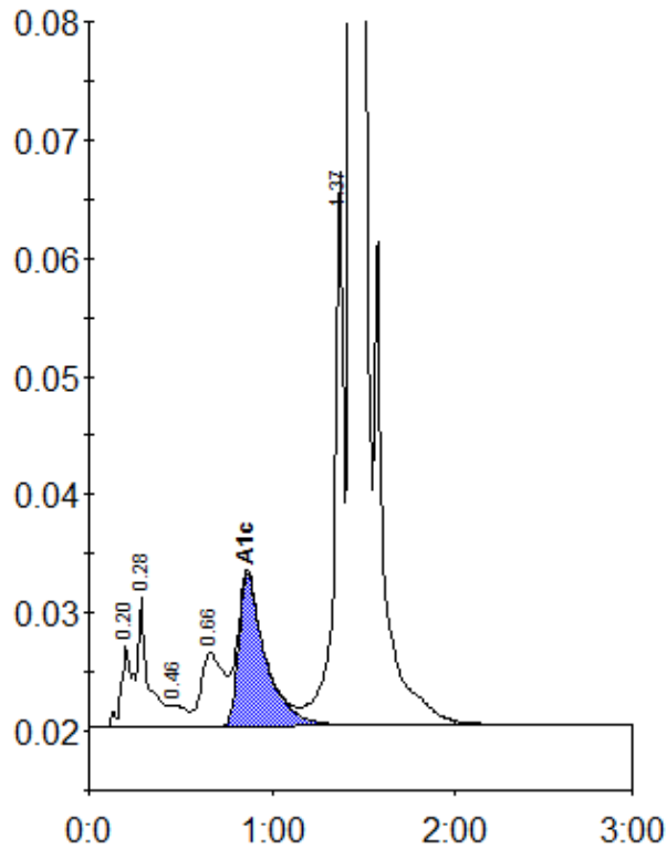
Peak table - ID: 11649805
