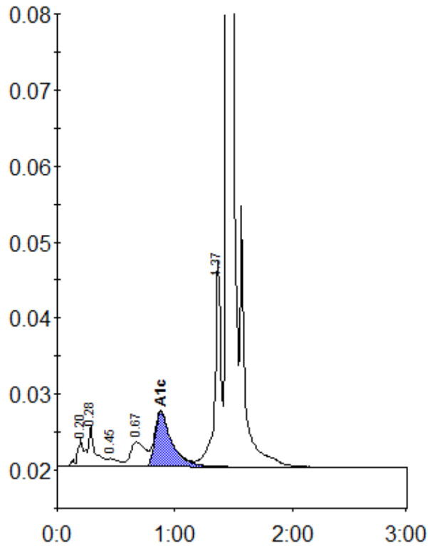
Peak table - ID: 11635408
