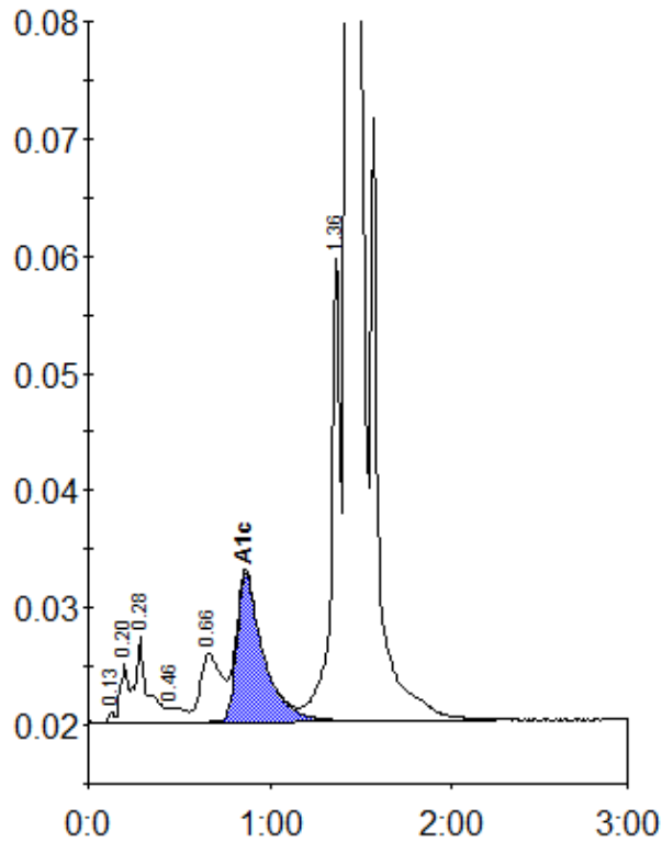
Peak table - ID: 11639087
