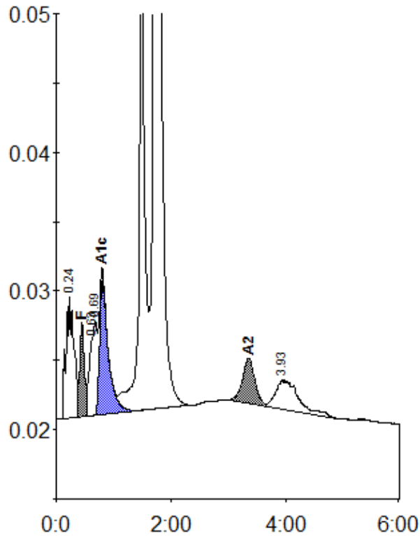
Peak table - ID: 11408020
