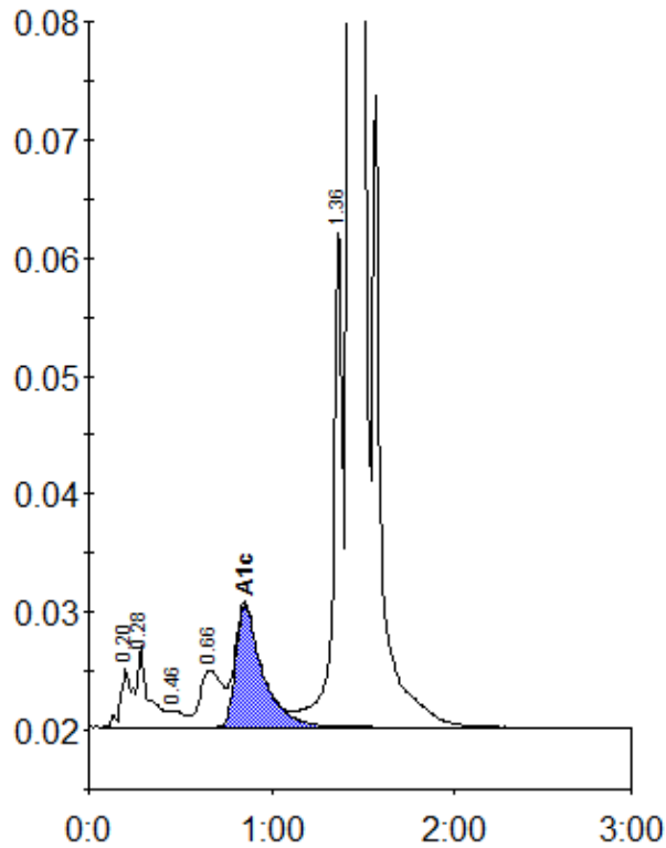
Peak table - ID: 11496235
