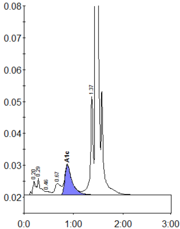
Peak table - ID: 11479076
