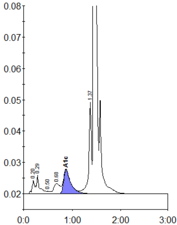
Peak table - ID: 11518503
