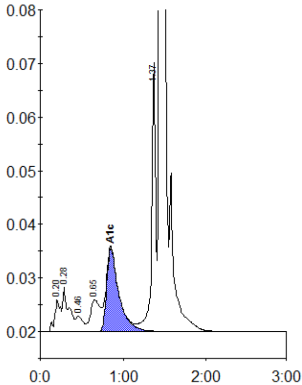
Peak table - ID: 11581012
