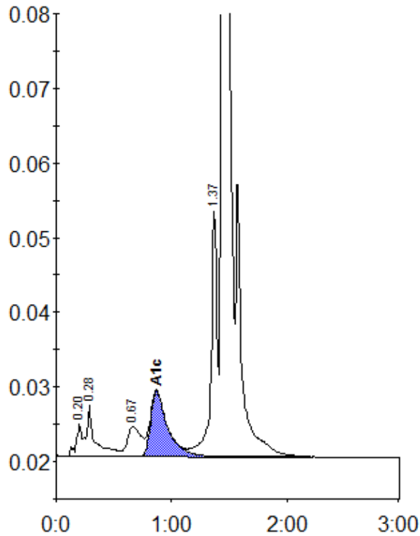
Peak table - ID: 11489337
