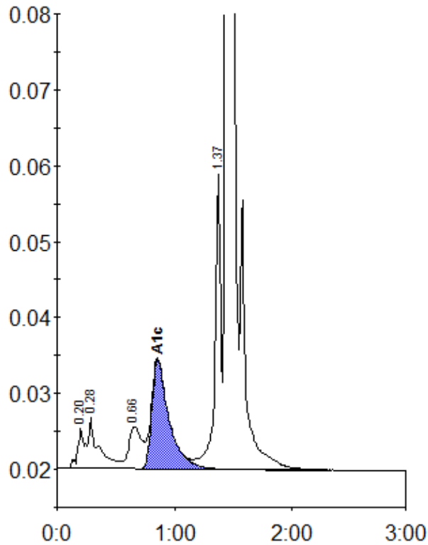
Peak table - ID: 11475642
