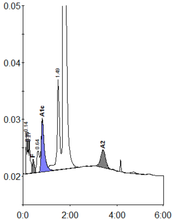
Peak table - ID: 11637596
