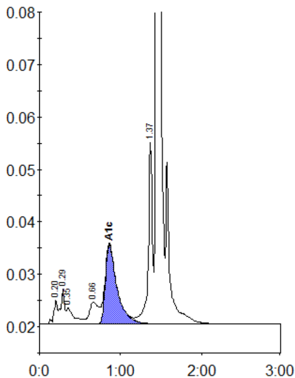
Peak table - ID: 11478334
