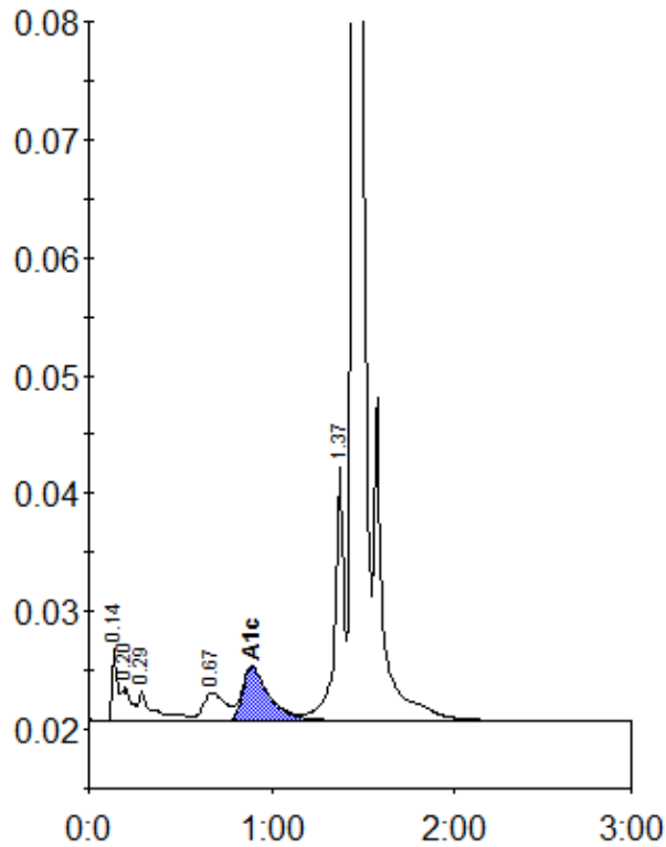
Peak table - ID: 11528849
