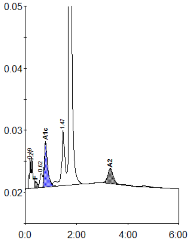
Peak table - ID: 11517186
