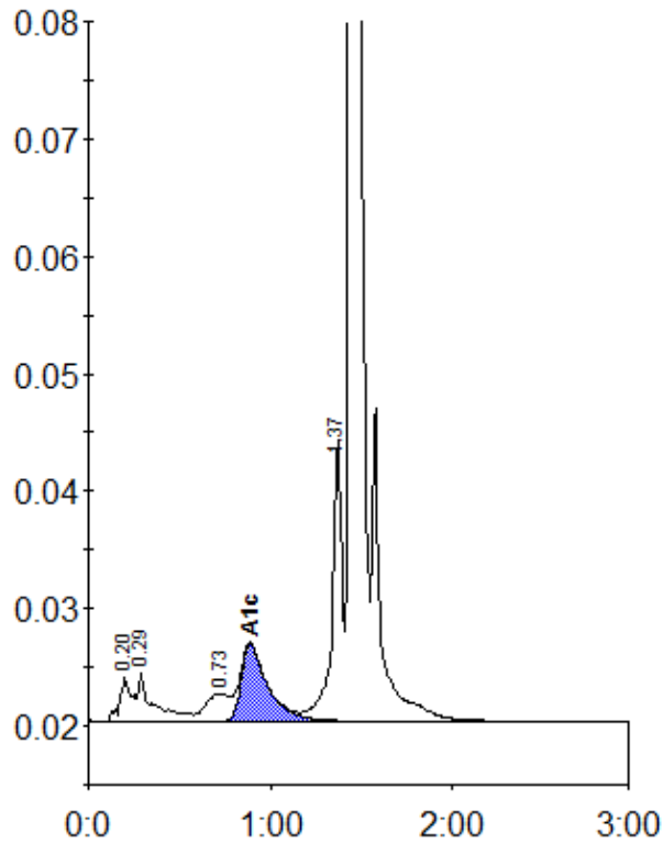
Peak table - ID: 11056459
