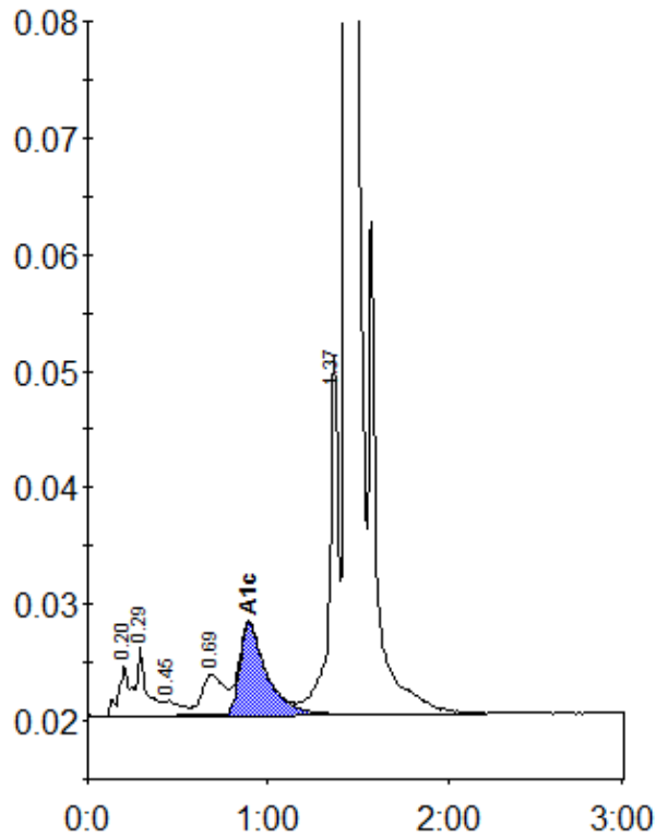
Peak table - ID: 11480278
