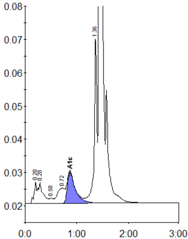
Peak table - ID: 11527743
