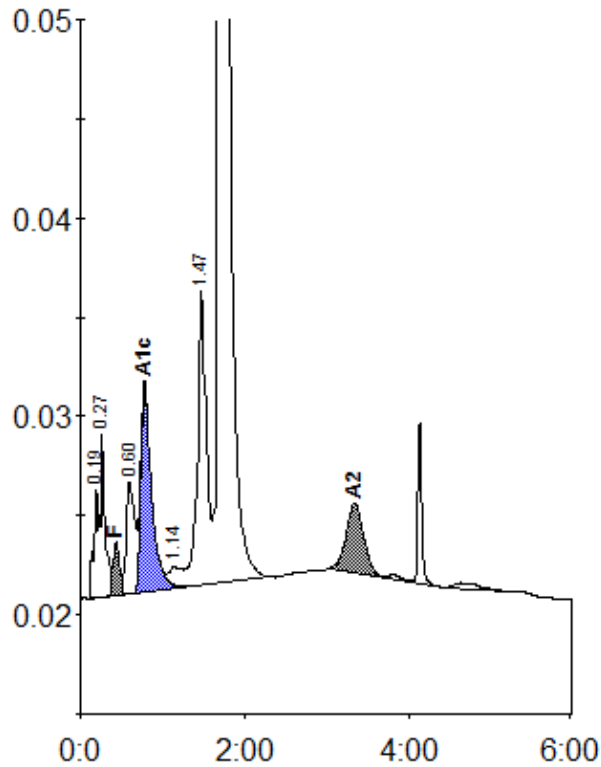
Peak table - ID: 11508792
