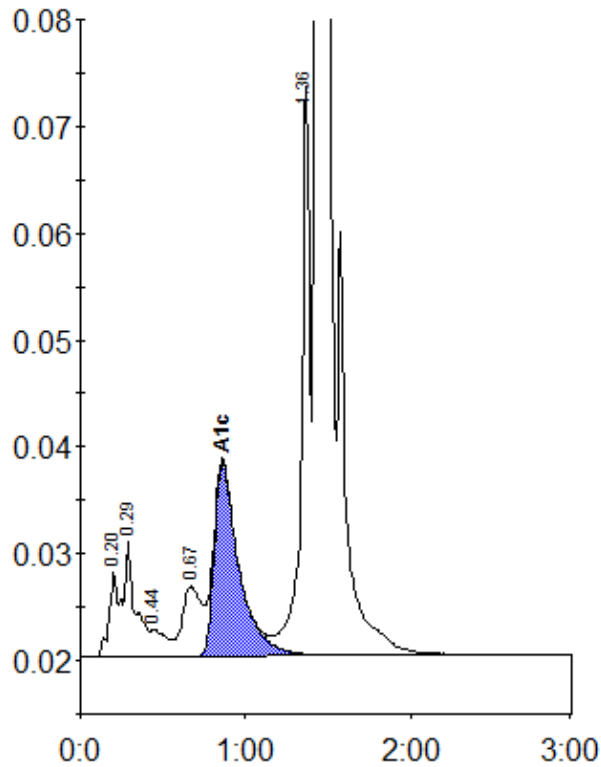
Peak table - ID: 11531810
