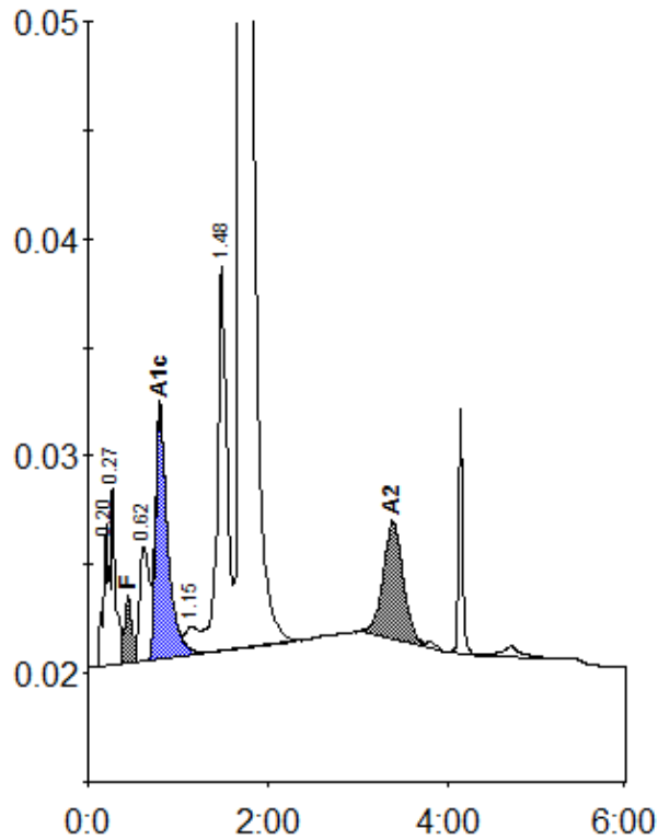
Peak table - ID: 11531883
