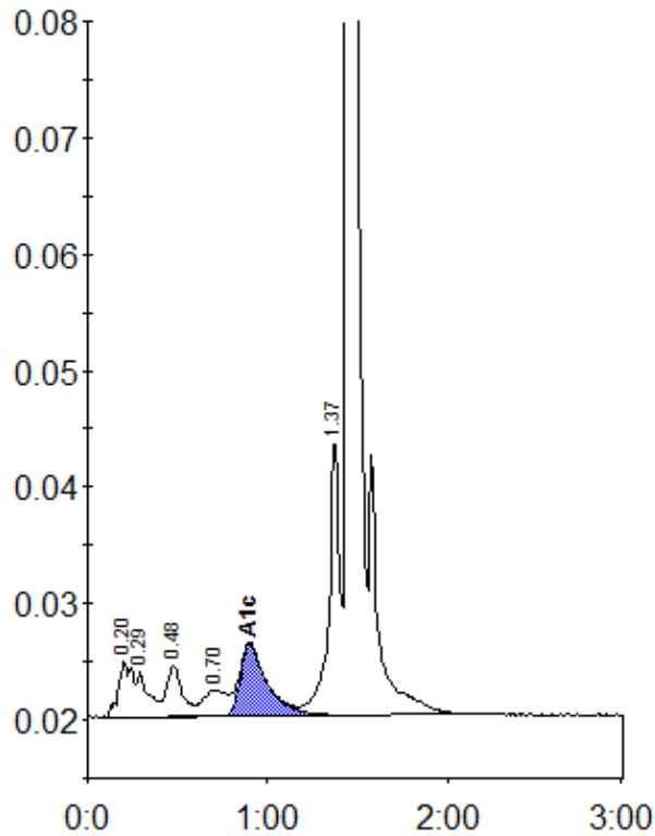
Peak table - ID: 11527963
