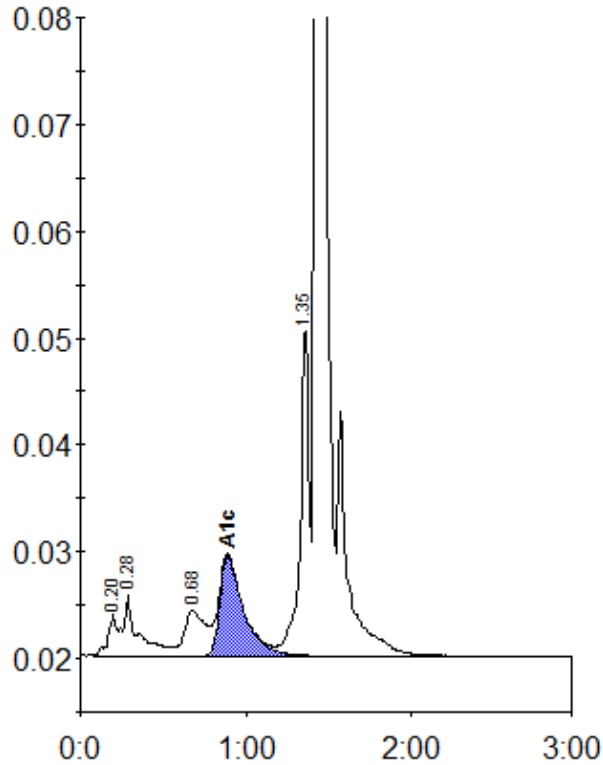
Peak table - ID: 11590451
