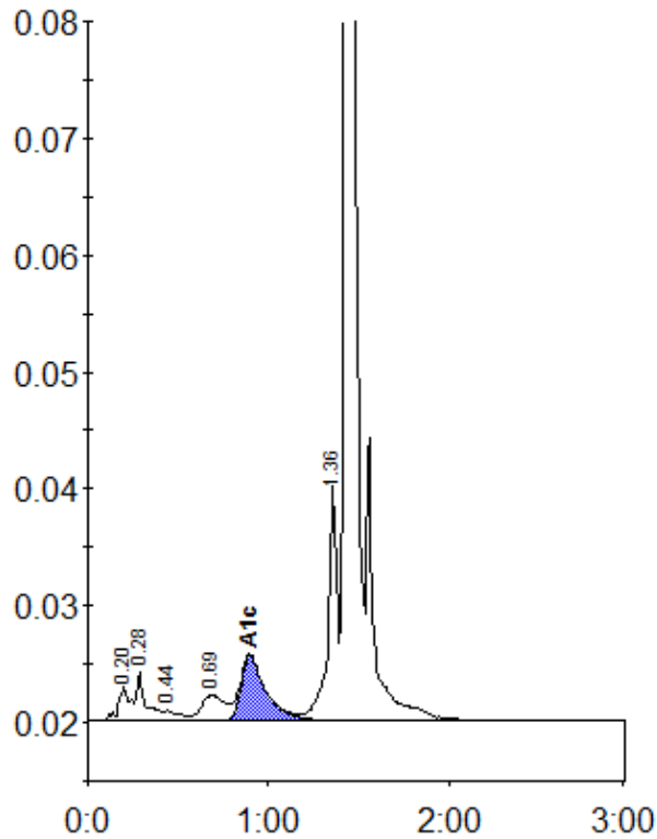
Peak table - ID: 11500789
